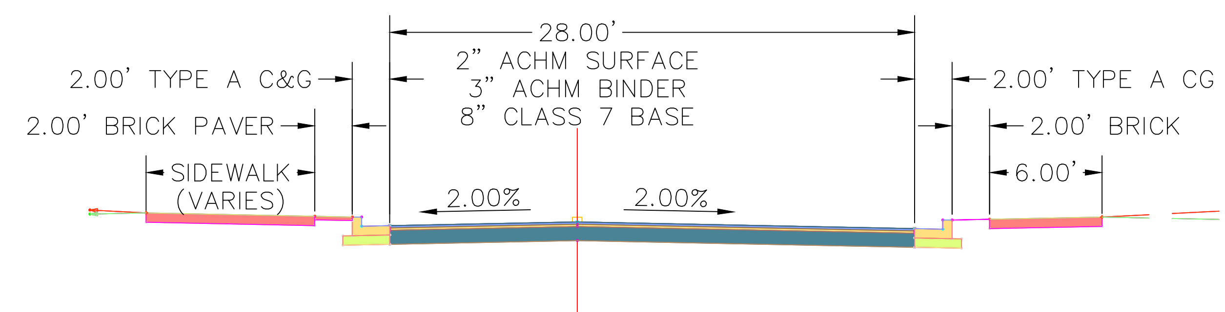
Spencer Street Typical Section (with parking)
