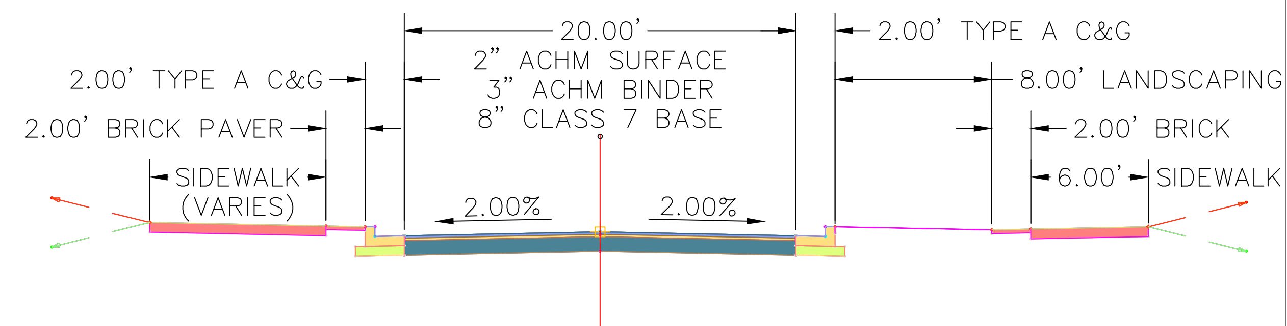
Spencer Street Typical Section
