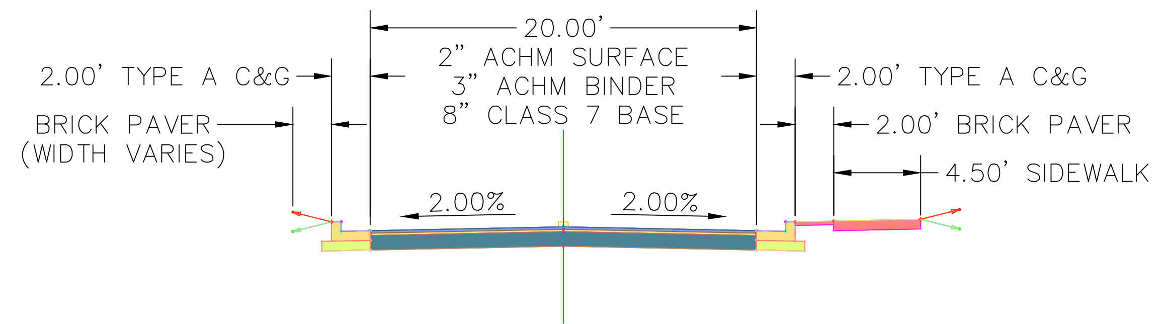
West Smith Street Typical Section
