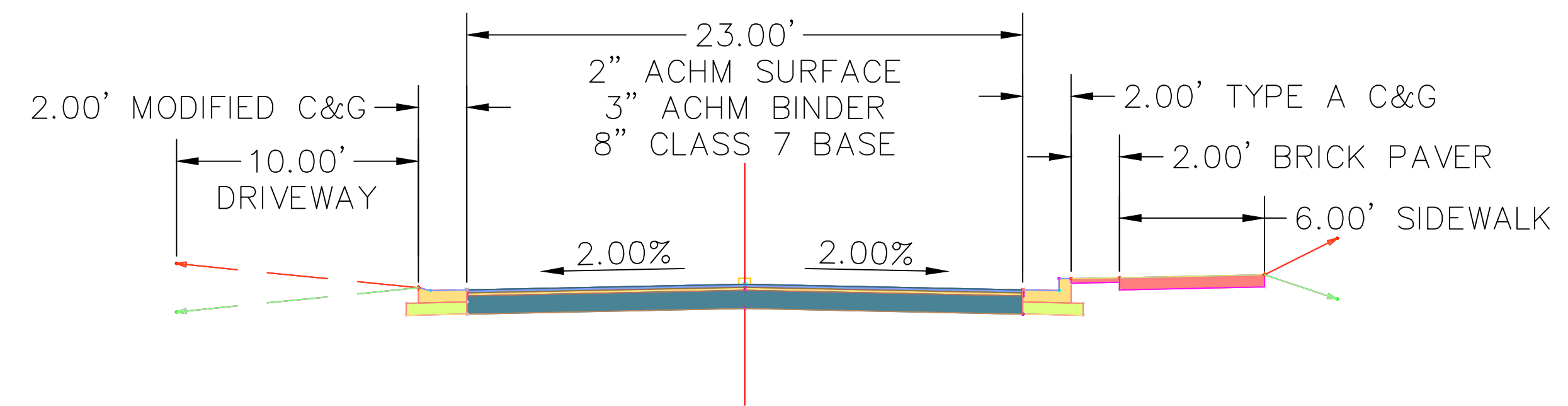
East Smith Street Typical Section
