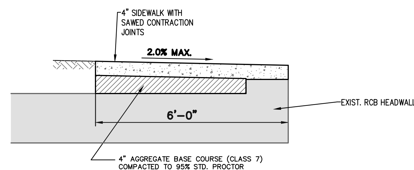
SIDEWALK SECTION AT RCB HEADWALL NTS
