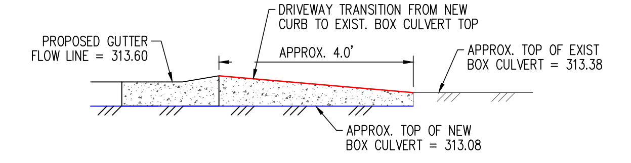
DRIVEWAY TRANSITION DETAIL
