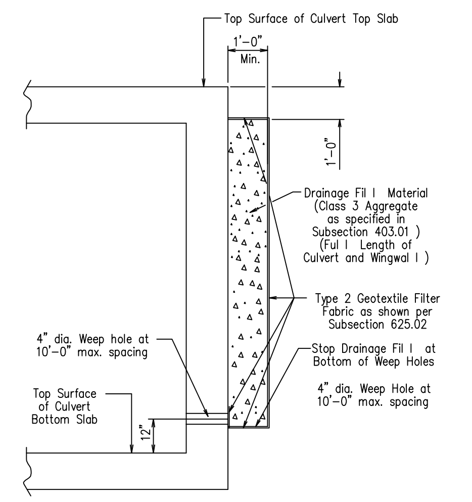
CULVERT DRAINAGE DETAIL
